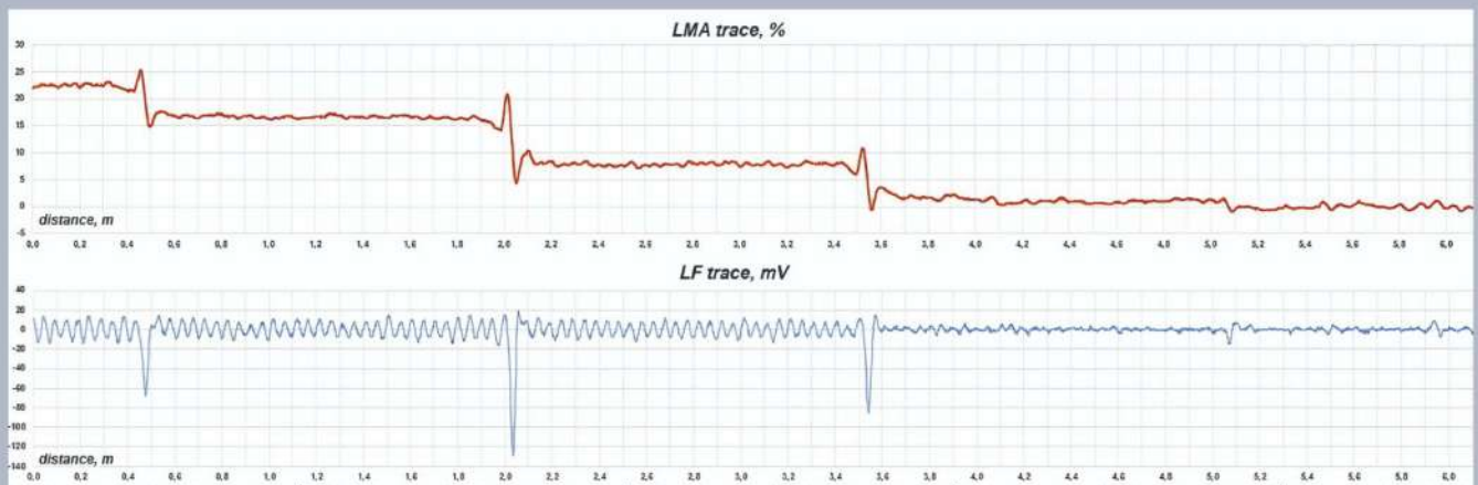
Example of data obtained during inspection of 24 mm diameter wire rope with the local faults
