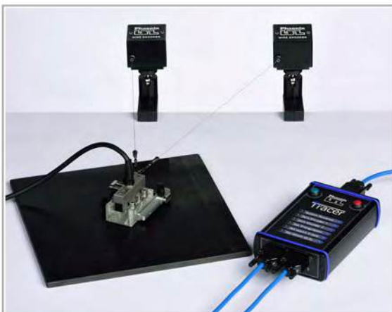
Tracer Set-Up
